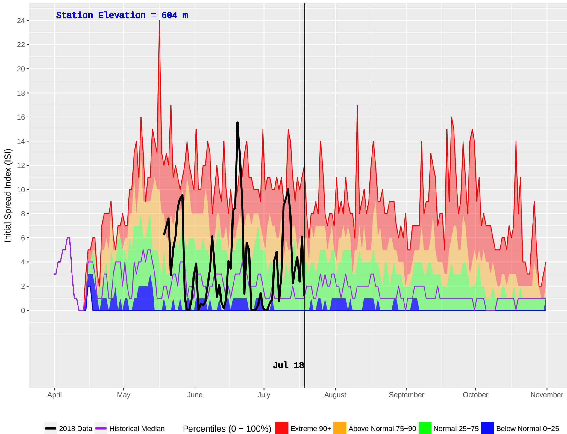
NELSON FORKS (119) : Historical (1986–2016) and Current (2018) Daily Initial Spread Index (ISI)
