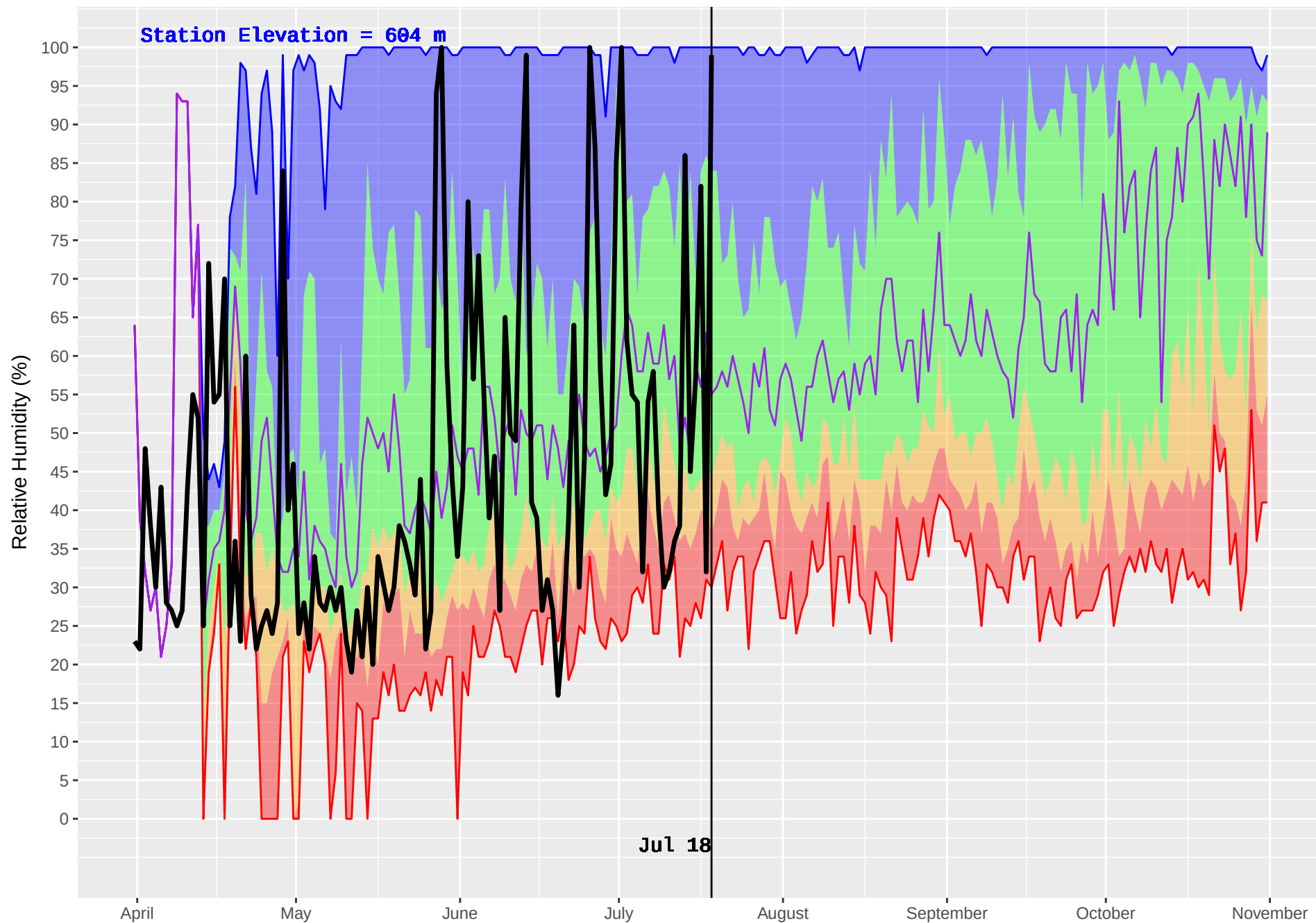
NELSON FORKS (119) : Historical (1986–2016) and Current (2018) Daily Relative Humidity
